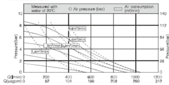
Performance curve
